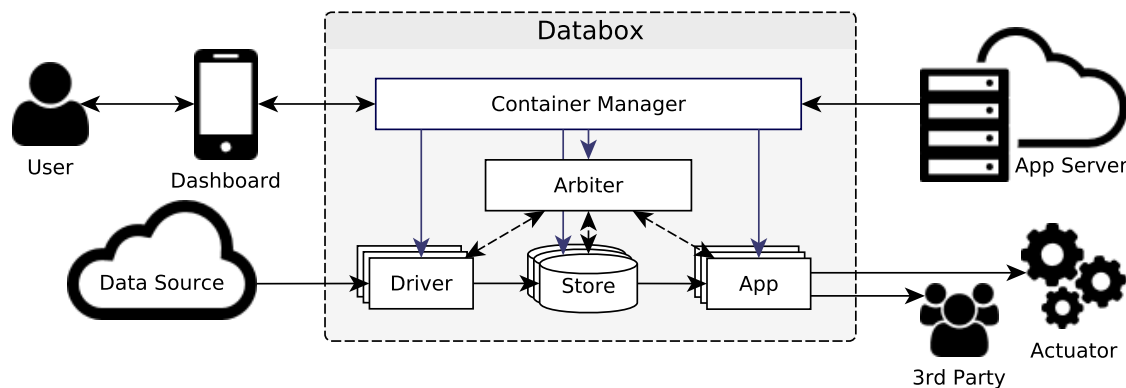
Figure 1: A High-level Overview of Databox Components
