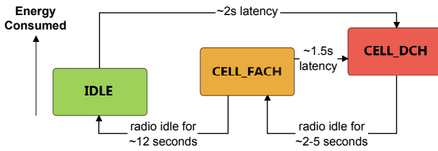
Figure 11: A common 3G wireless RRC state machine.
